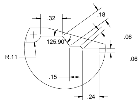
DETAIL E
