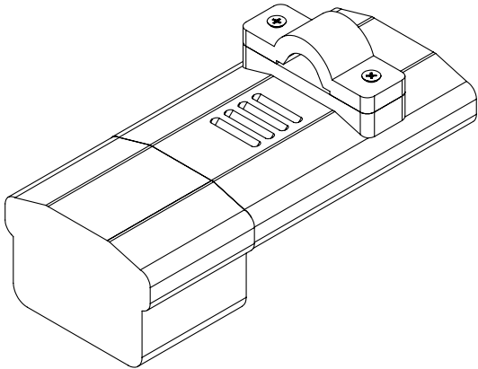
LOGGER ENCLOSURE ASSEMBLY ISOMETRIC VIEW
