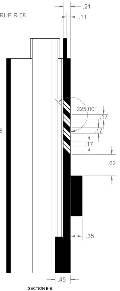
SECTION B-B
